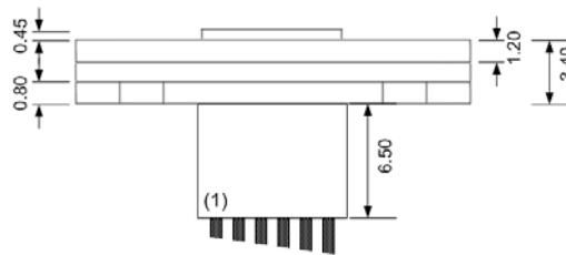
Fig 12. Side view
