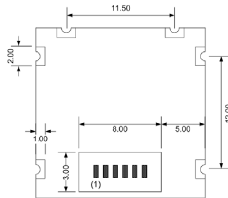
Fig 11. Bottom view
