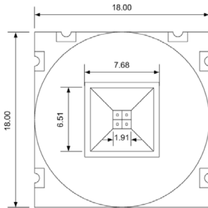
Fig 10. Top view
